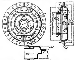
Figs. 931-933. Cast Steel Back Cylinder Head. American Locomotive Co.
